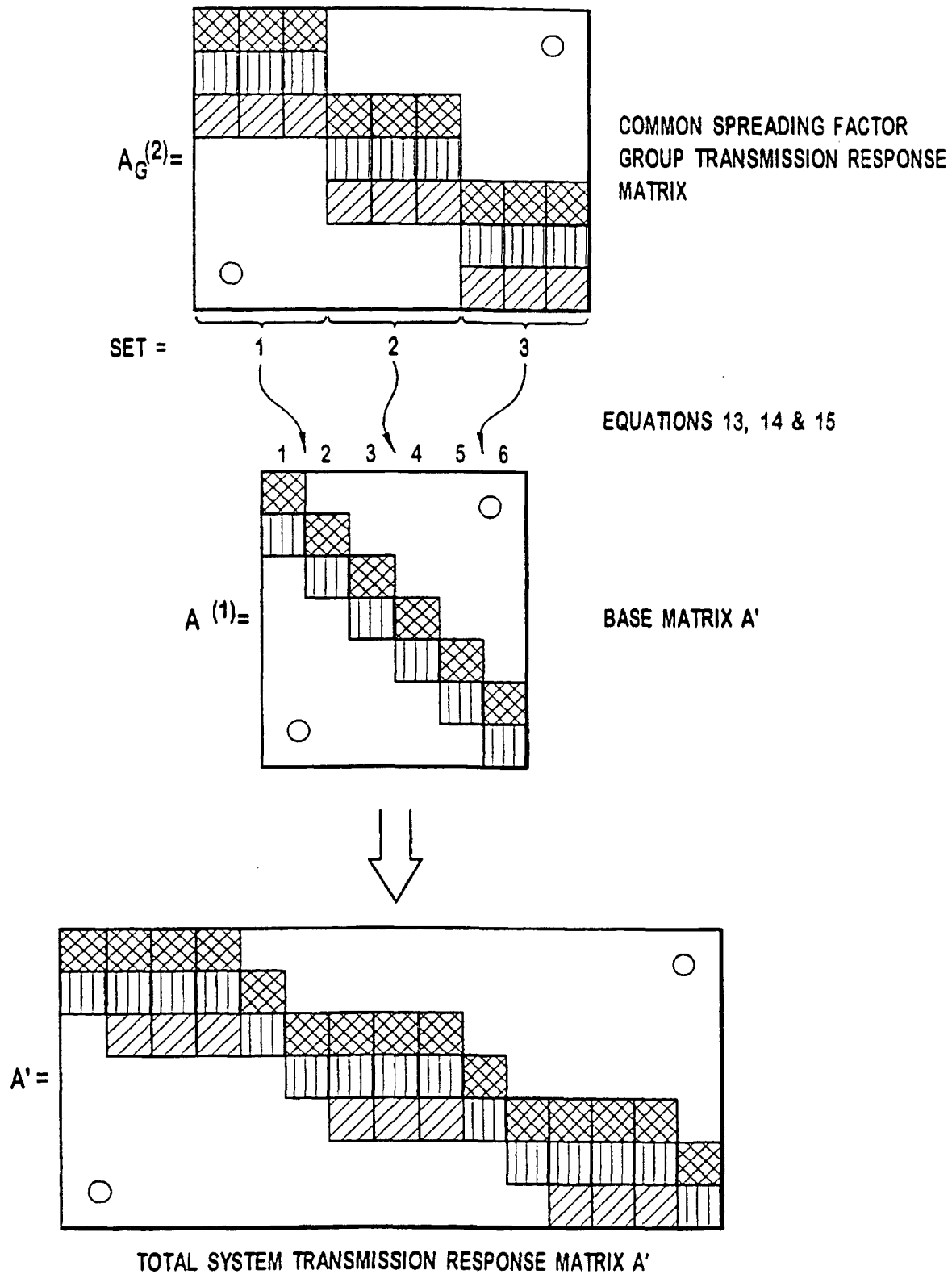
ASSEMBLY FIG. 12
