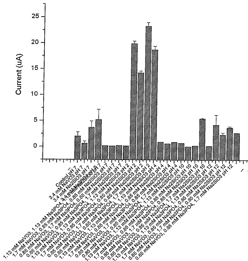
Ternary Combinations of Sodium Metavanadate, Sodium Metasilicate, and Sodium Phosphate evaluated using Polarization Method
