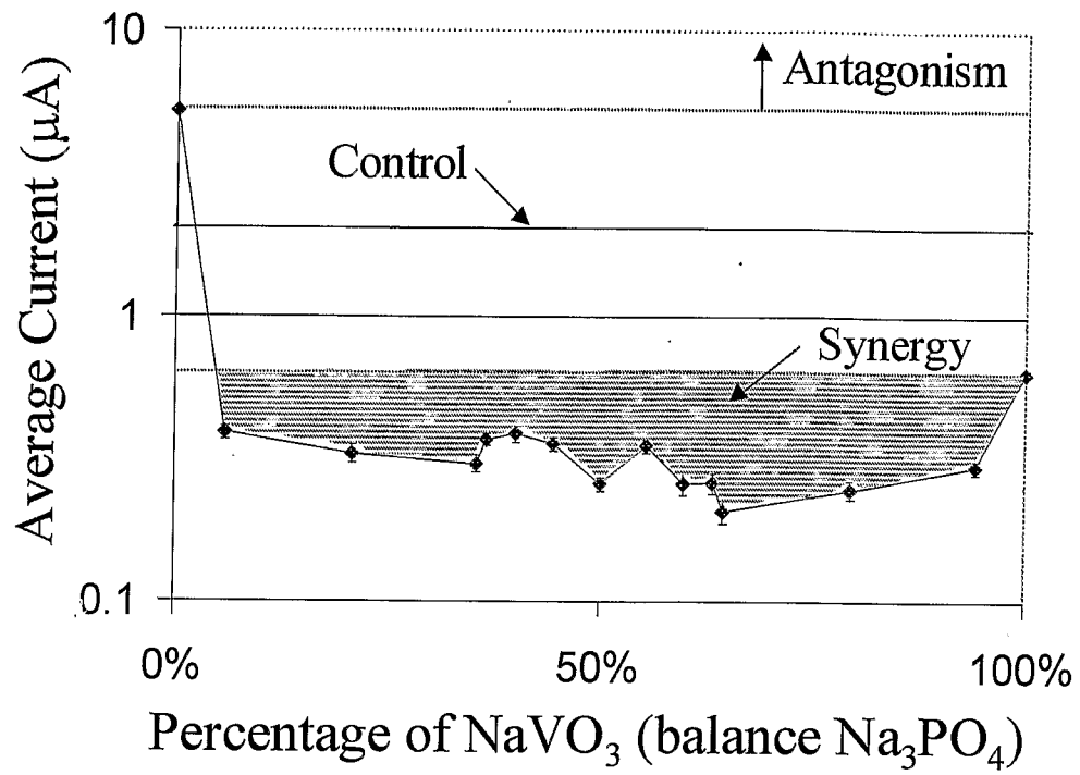
Figure 9. Plot of current of 3.4 mM NaVO 3 /Na 3 PO 4 , 0.6 M NaCl (pH 7)
