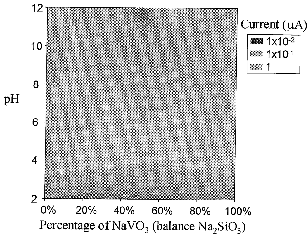
Figure 11. Current from MMA testing of 3.4 mM NaVO 3 /Na 2 SiO 3 varying pH 2-12.
