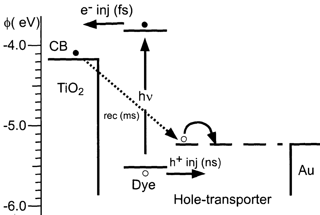
Figure 2 - Schematic representation of charge transfers taking place in DSC operation.
