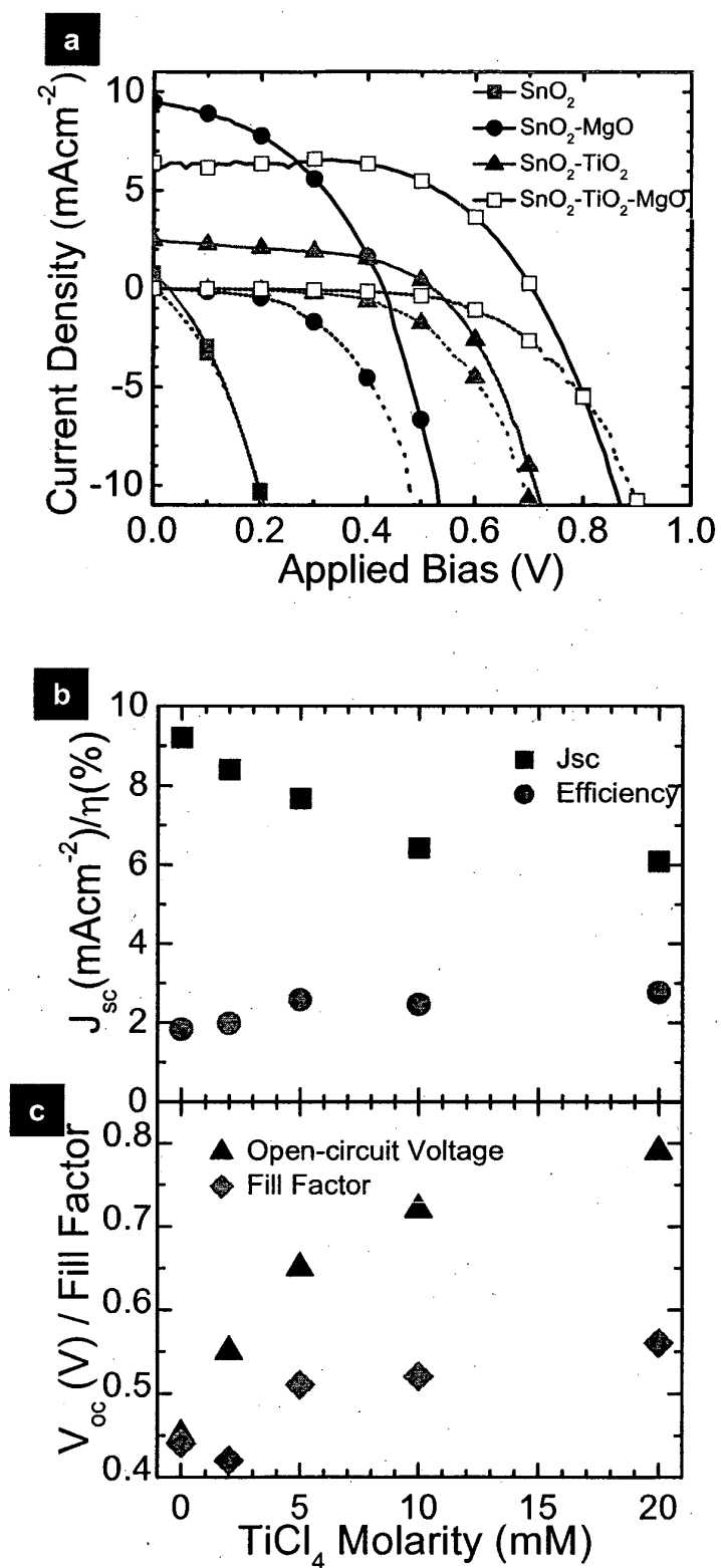
Figure 3. Performance of \text{SnO}_2 -based SDSCs
