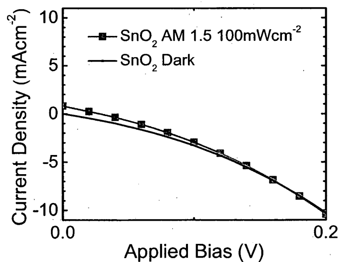
Figure 7 - . Performance of a comparative SDSC formed with bare \text{SnO}_2 having no surface coatings. Device structure: FTO/compact \text{SnO}_2 /mesoporous \text{SnO}_2 /dye/p-type hole-transporter/silver.
