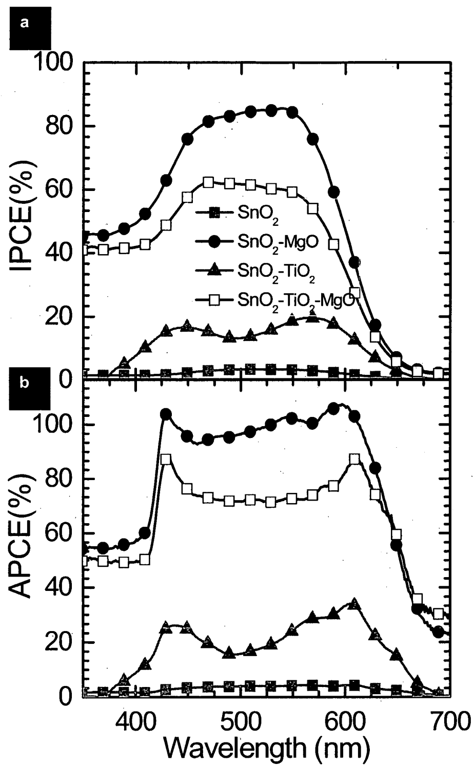
Figure 4. Light absorption characteristics of SnO 2 -based SDSCs
