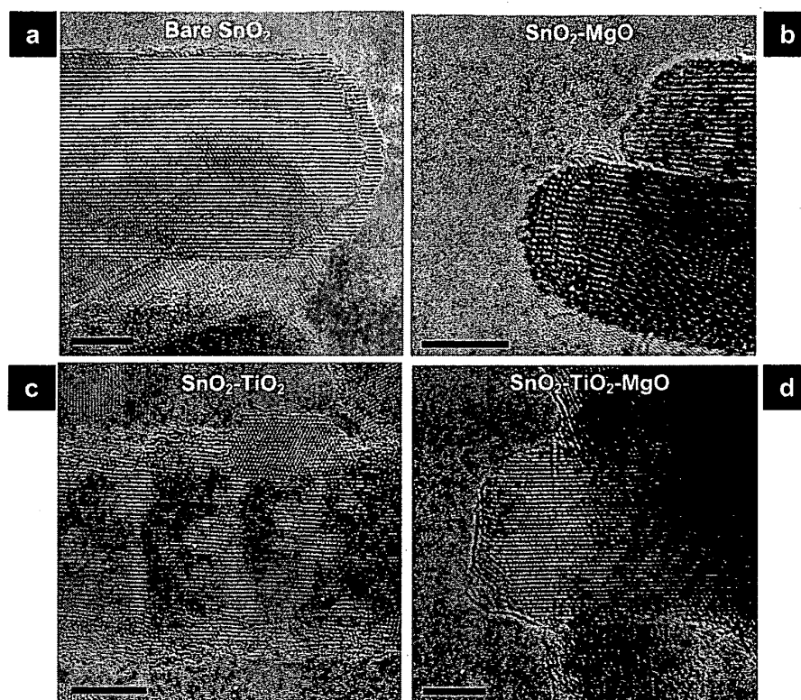
Figure 6 - HRTEM images of \text{SnO}_2 films uncoated and coated for use in accordance with the present invention.
