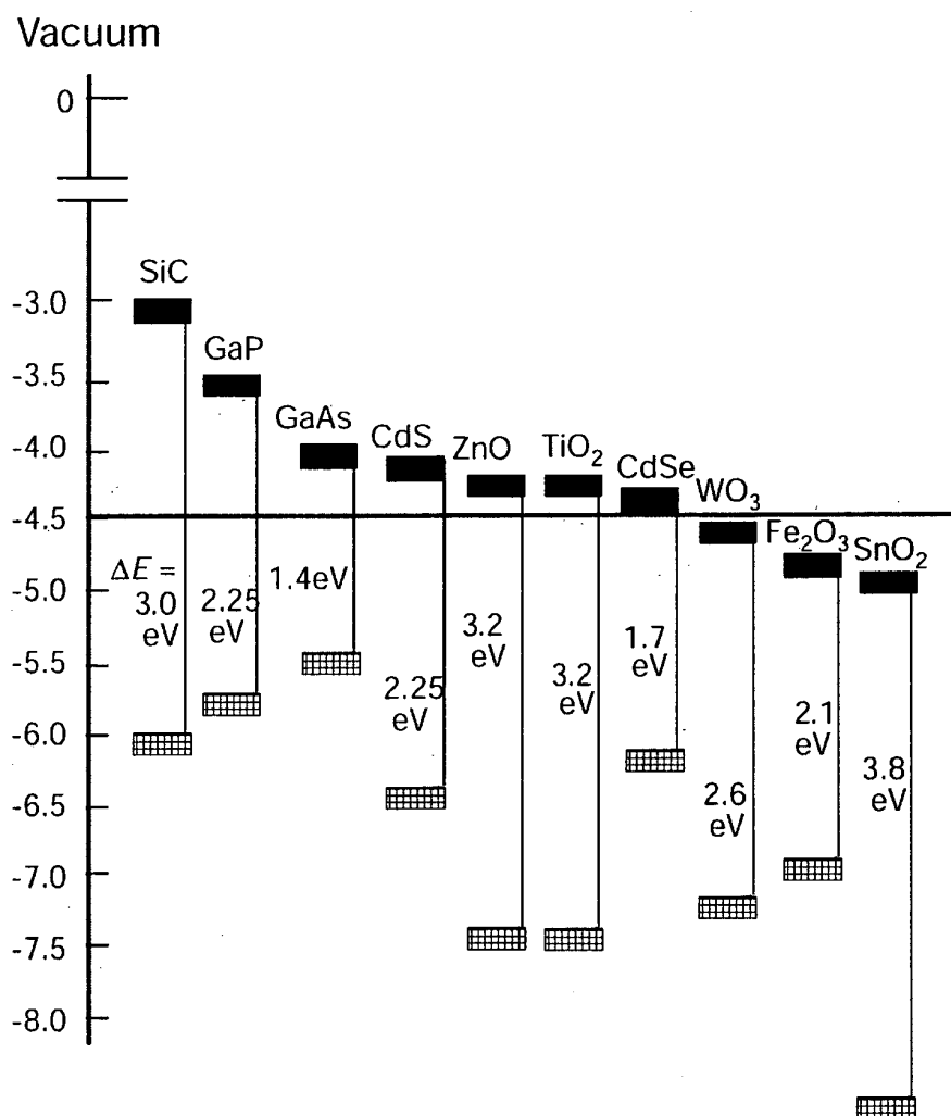
Figure 9 - Graphical representation of band gap and conduction bands in typical semiconductor materials useful in the present invention.
