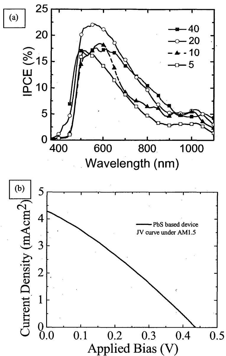
Figure 8. Spectral response (top) and current voltage curve (bottom) measured under AM 1.5 simulated sun light at 100 \text{ mW cm}^{-2} intensity for a \text{SnO}_2\text{-MgO} / PbS QD/ Spiro-OMeTAD based solar cell.
