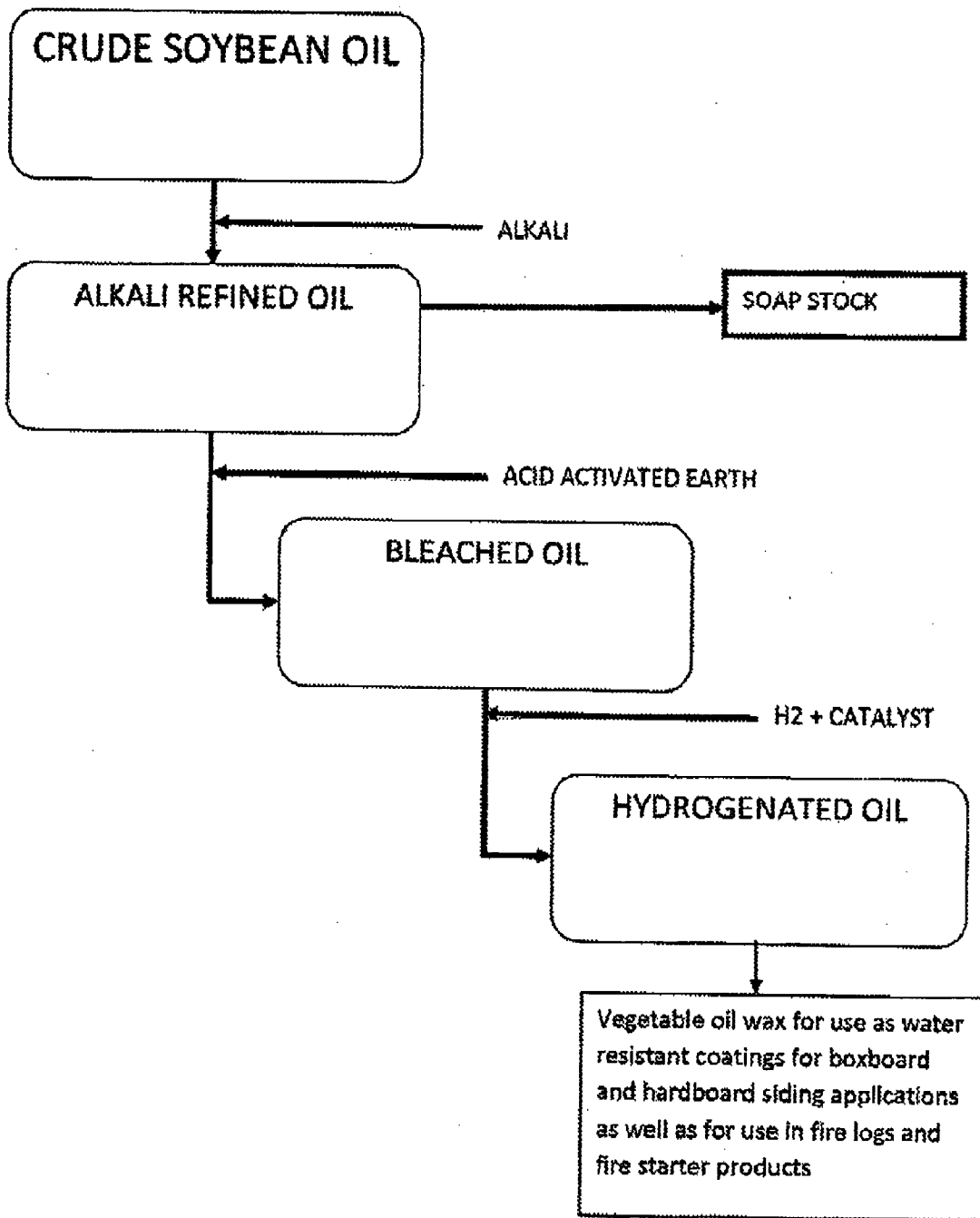
Figure 2 . Modified Renewable Oil processing without Degumming & Deodorizing
