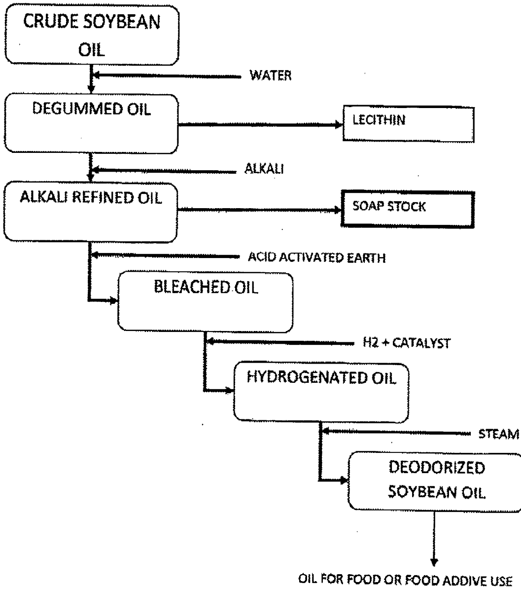
Figure 1 Conventional Renewable oil processing
