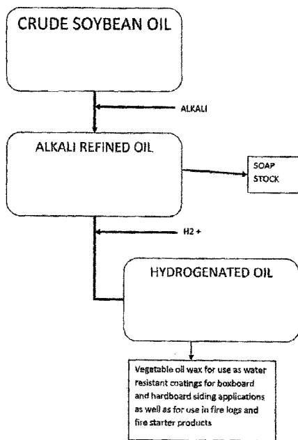
Figure 3. Modified Renewable Oil processing without Degumming, Bleaching and & Deodorizing
