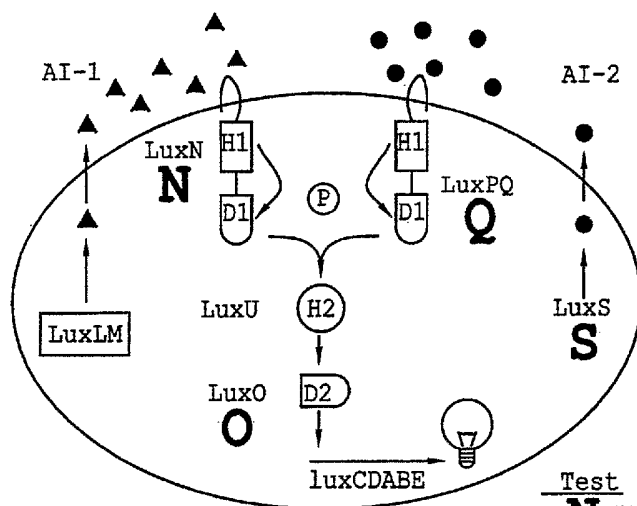
Hybrid quorum sensing circuit of Vibrio harveyi
