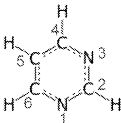
Pyrimidine
