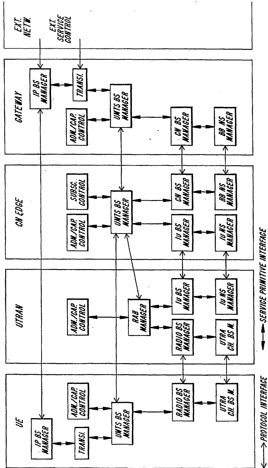
Fig. 16 PRIOR ART
