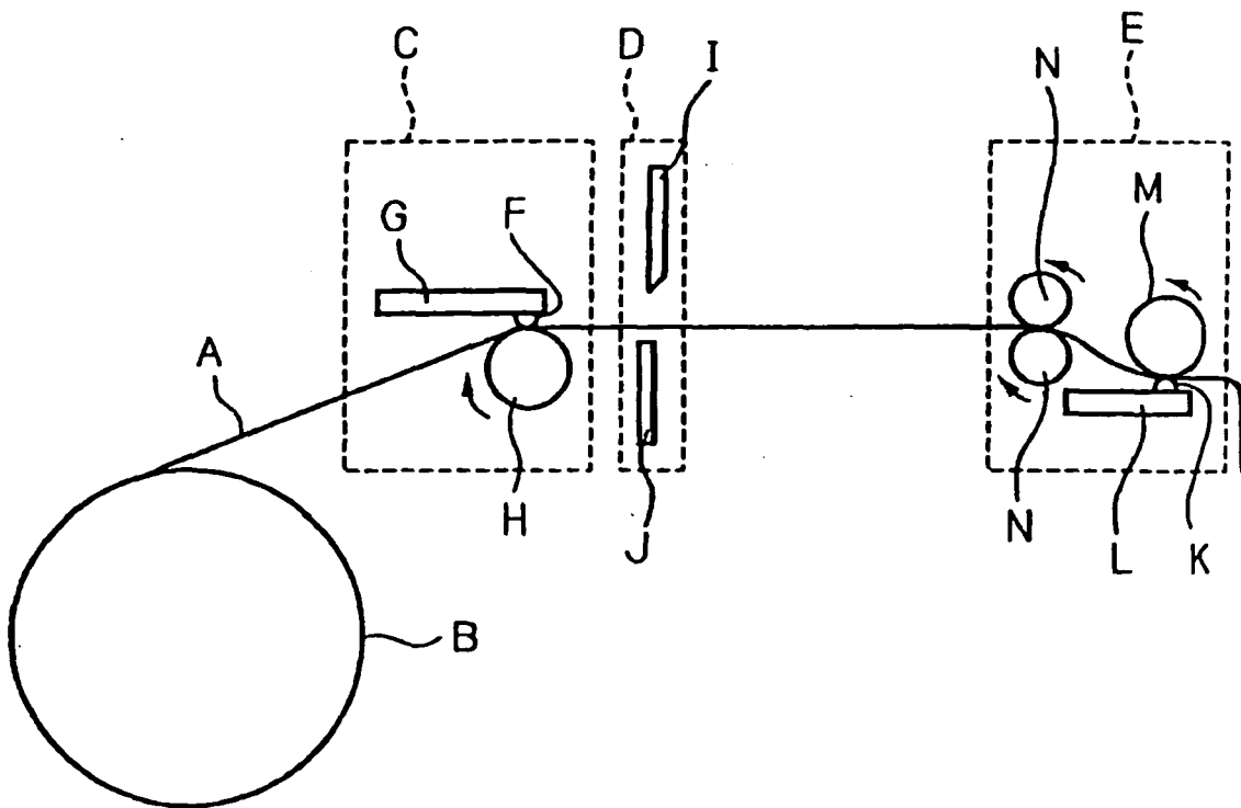
FIG. 4 PRIOR ART
