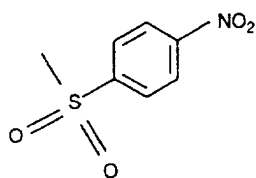
4-nitrophenylsulfonyl
