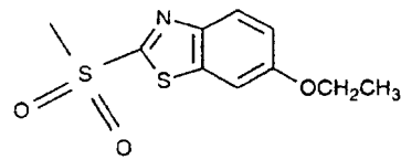
6-ethoxy-2-benzothiazolsulfonyl
