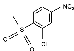
2-chloro-4-nitrophenylsulfonyl
