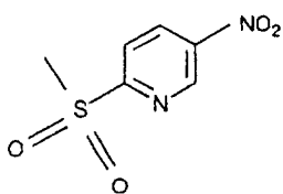
p-NO 2 -pyridinylsulfonyl
