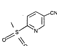
p-CN-pyridinylsulfonyl
