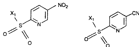
p-NO 2 -pyridinylsulfonyl
