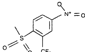
2-CF 3 -4-nitrophenylsulfonyl
