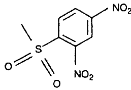
2,4-dinitrophenylsulfonyl
