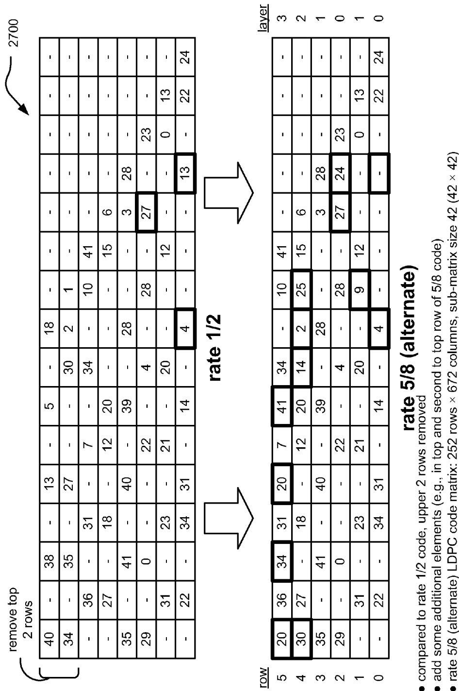
Fig. 27 (from rate 1/2 code to rate 5/8 code with sub-matrix size 42)
