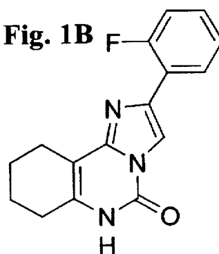
Compound 5
