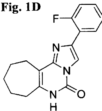
Compound 13
