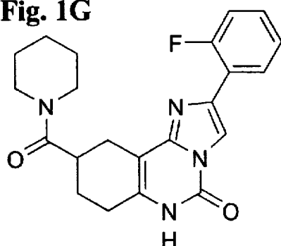
Compound 21
