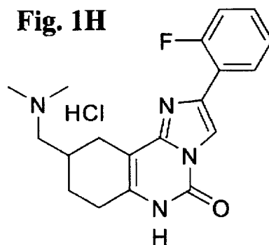
Compound 24
