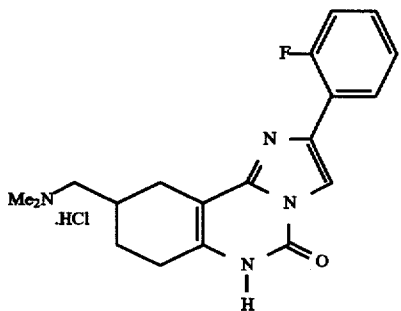
Compound 24
