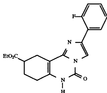
Compound 1
