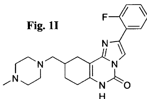
Compound 25
