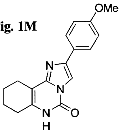
Compound 50
