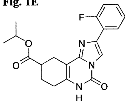
Compound 14
