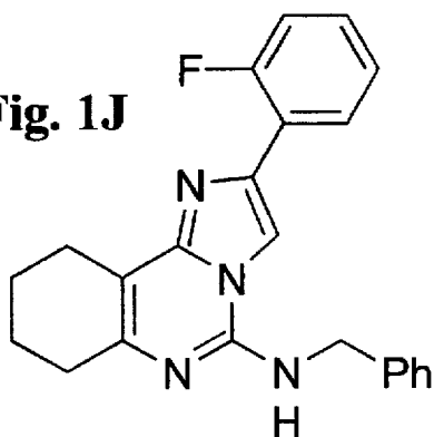
Compound 31
