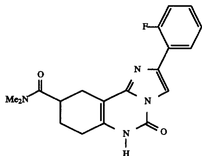
Compound 18
