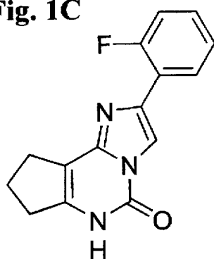
Compound 12
