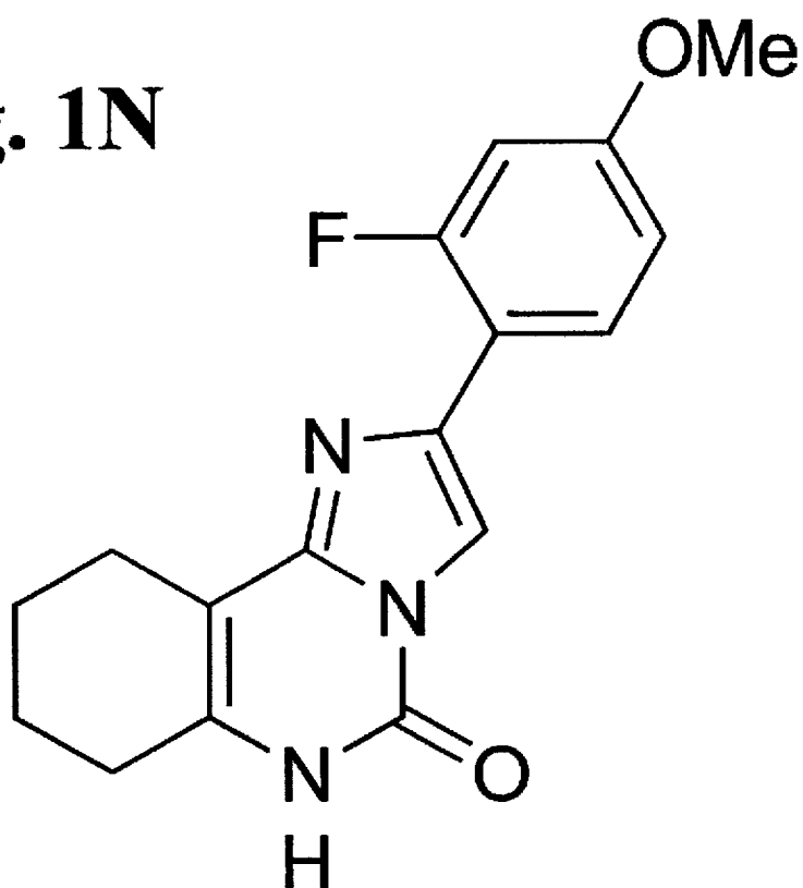
Compound 51
