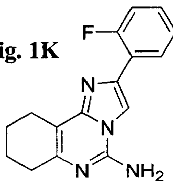
Compound 33
