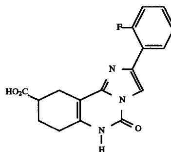
Compound 17
