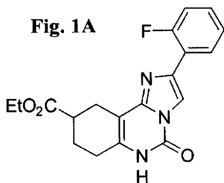
Compound 1
