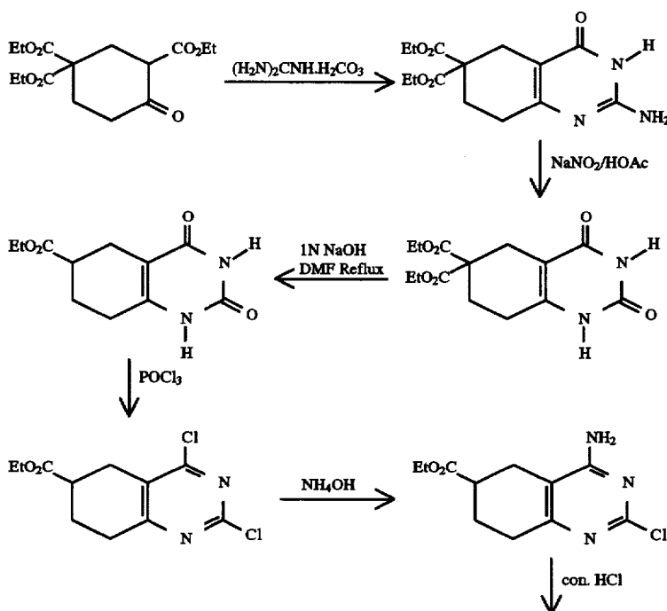
Scheme I
