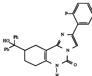
Compound 46
