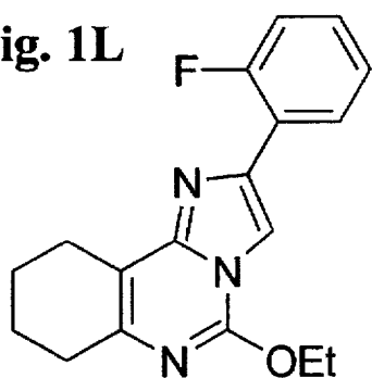
Compound 39
