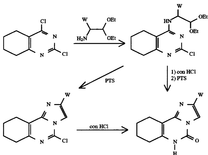
Scheme II
