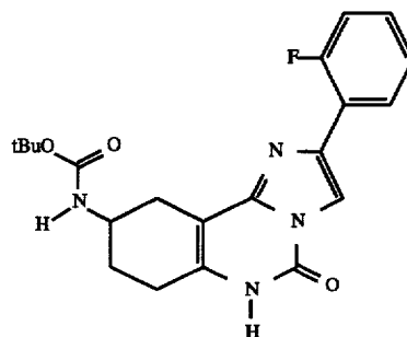
Compound 28
