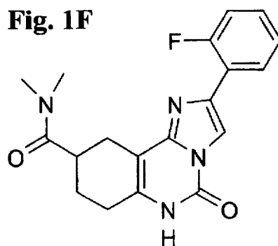
Compound 18
