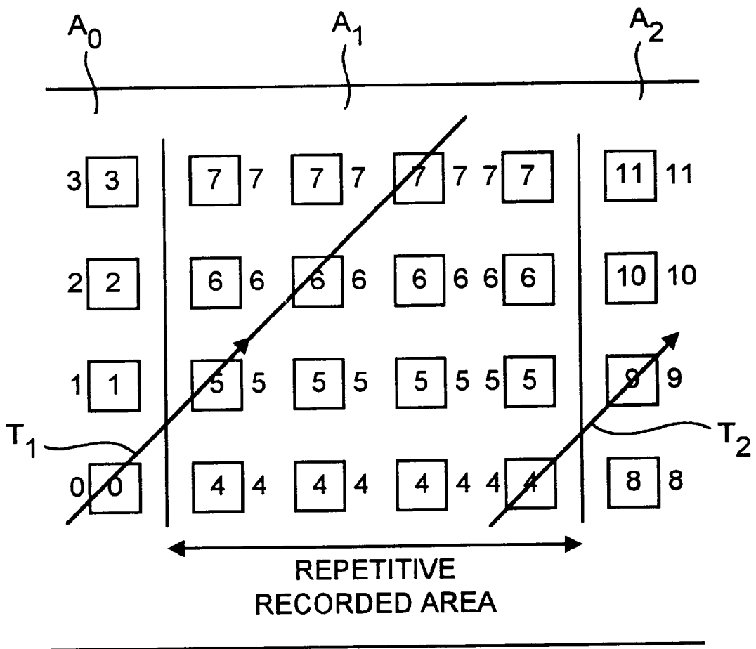
FIG. 8 (PRIOR ART)
