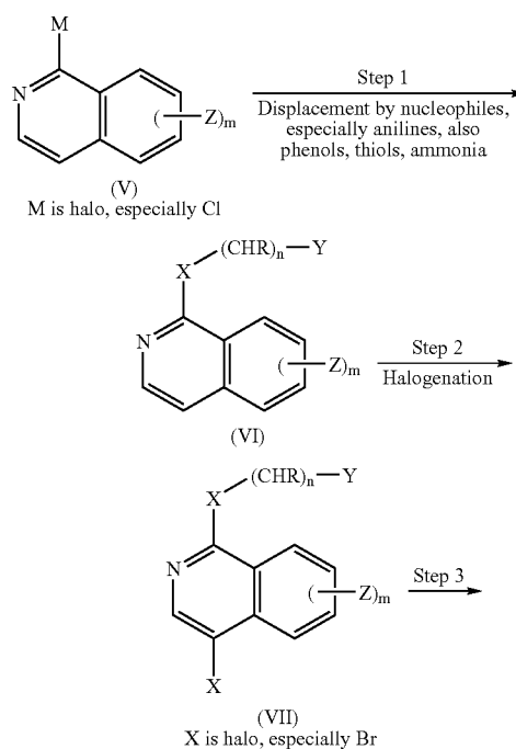
Suzuki Reaction Scheme
