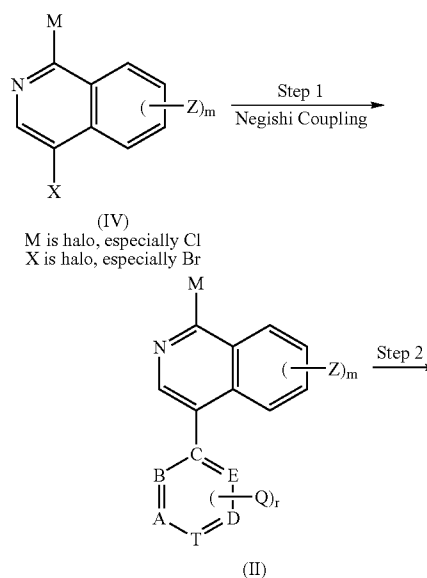
Negishi Reaction Scheme
