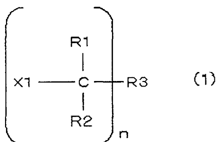
[Chemical Formula 1]
