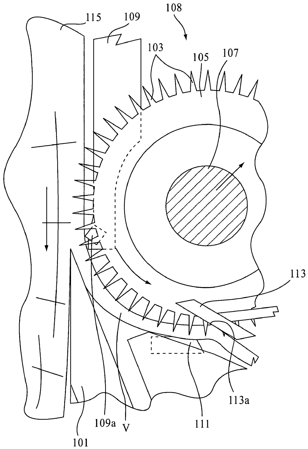
FIG. 18 PRIOR ART
