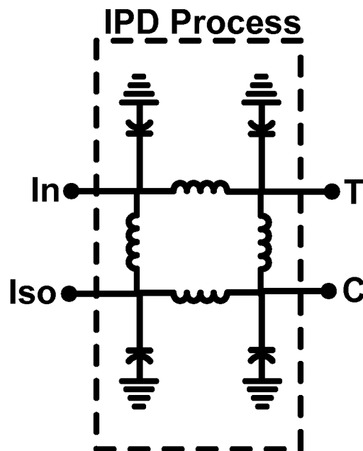
Lumped Branch Line Hybrid Coupler
