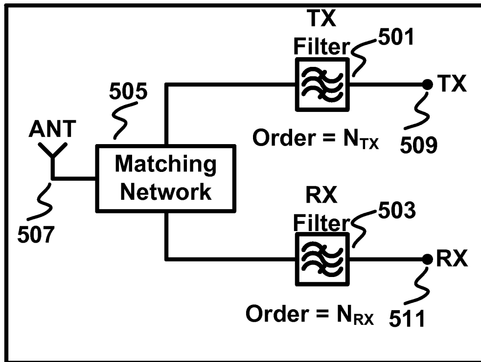
FIG. 5A (Prior Art) # of resonators = N_{TX} + N_{RX}
