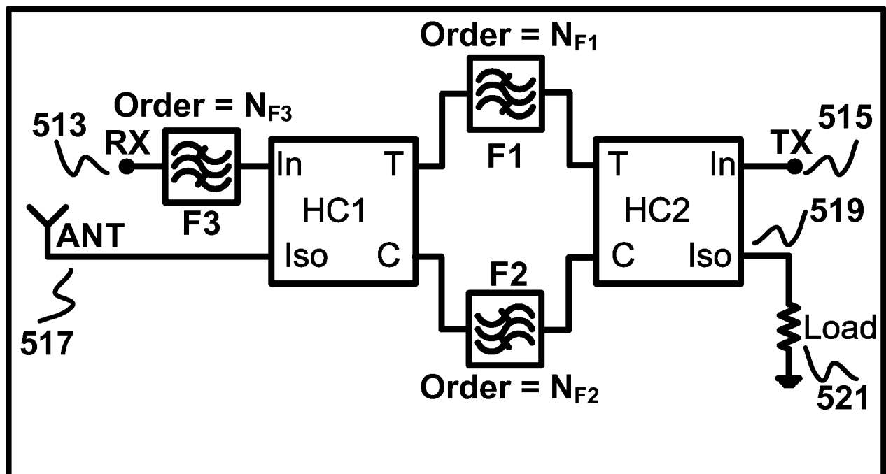
FIG. 5B # of resonators = N_{F1} + N_{F2} + N_{F3}
