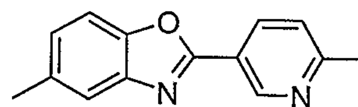
5-methyl-2-(6-methylpyridin-3-yl)-1,3-benzoxazole
