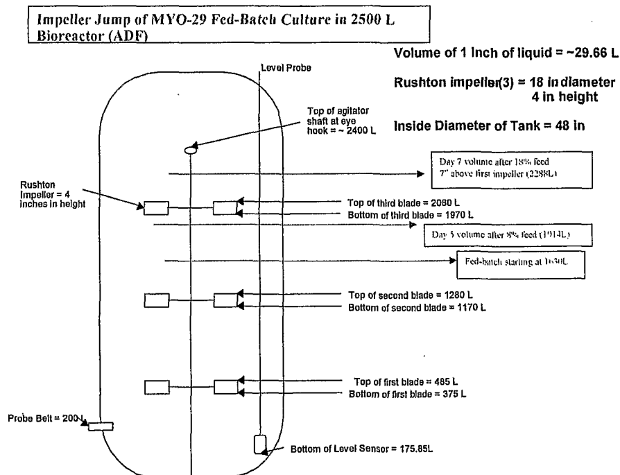
Figure 24. Impeller Jump
