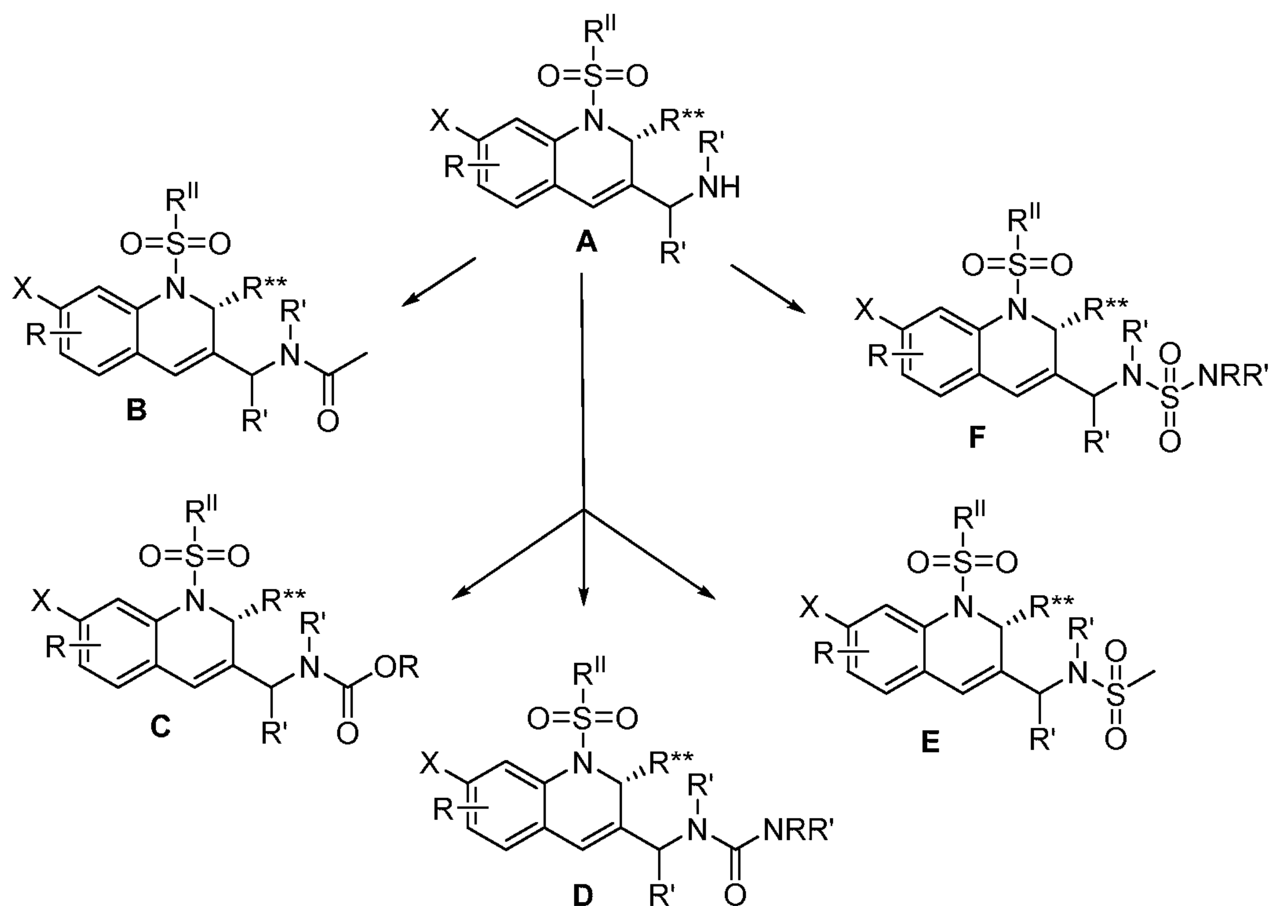
SCHEME 7.
