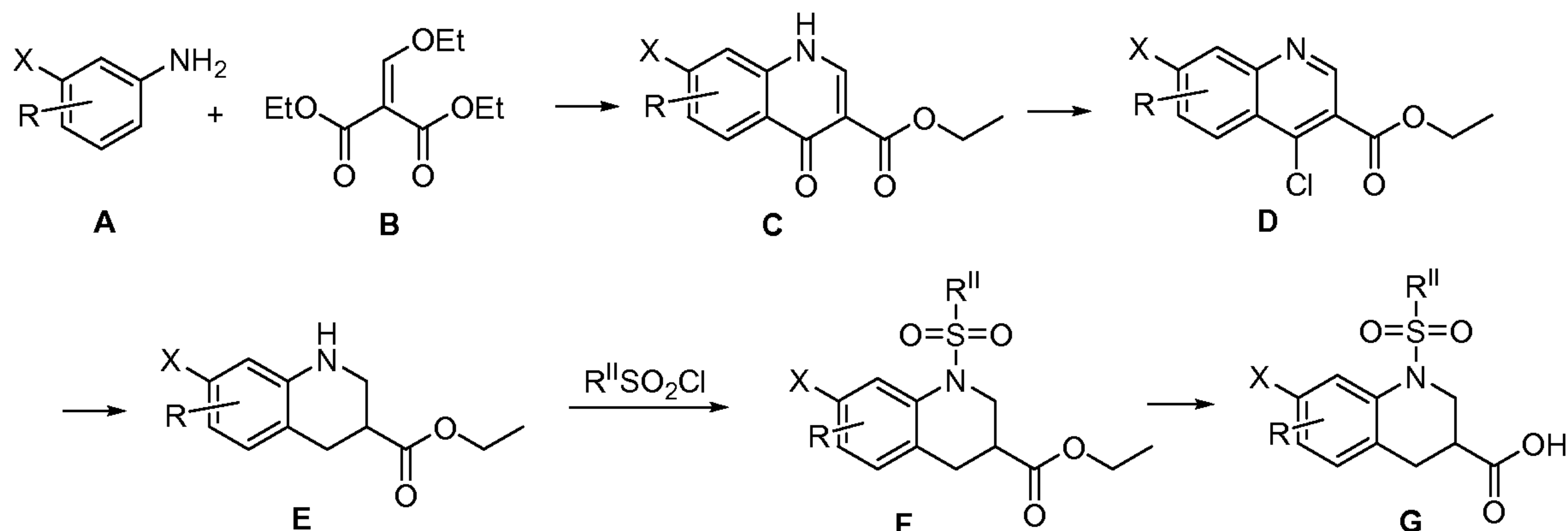
SCHEME 1.
