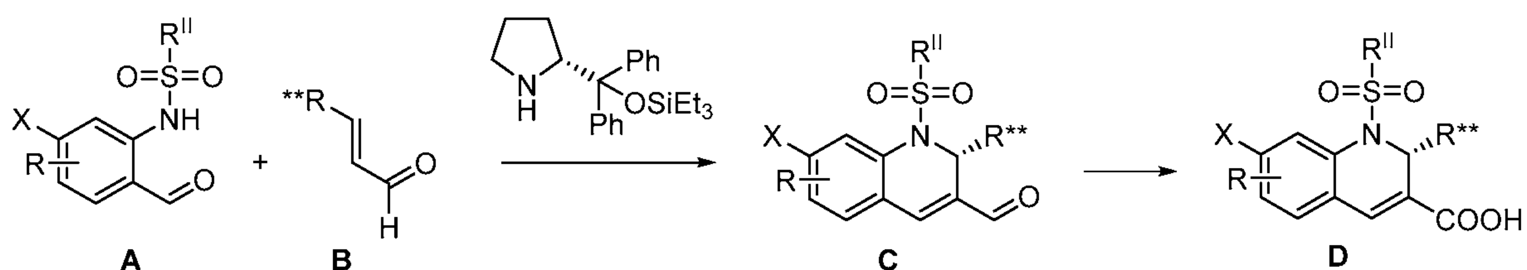
SCHEME 3.
