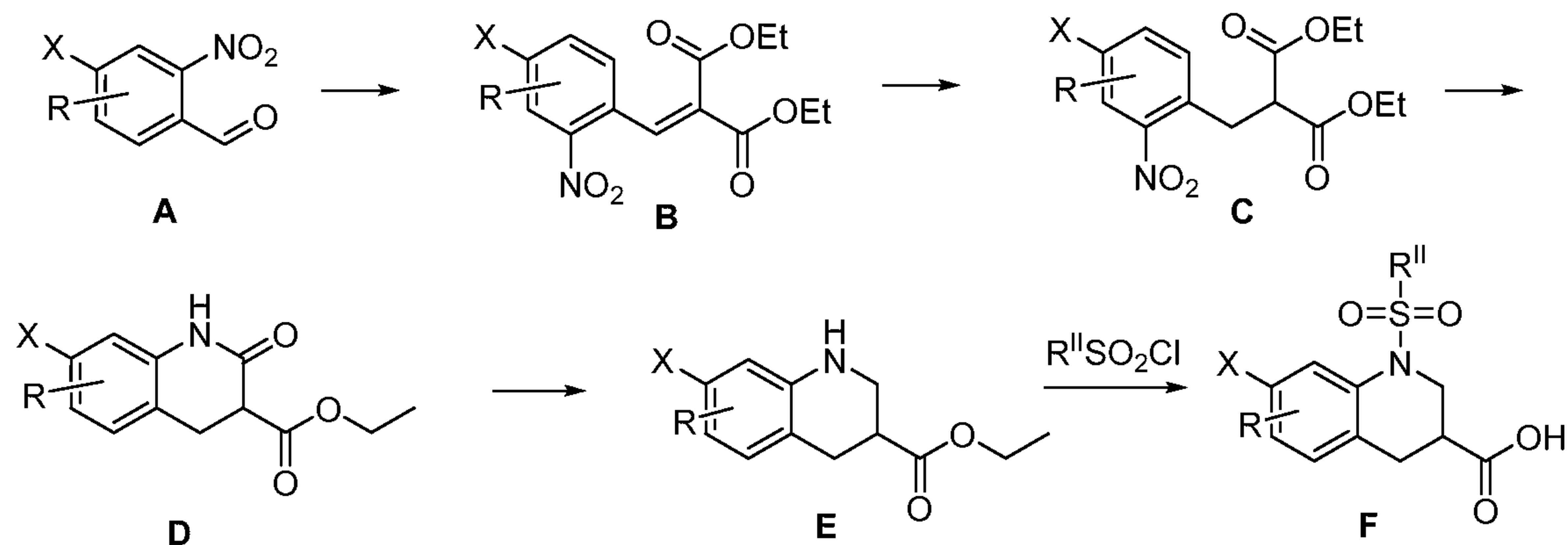
SCHEME 2.
