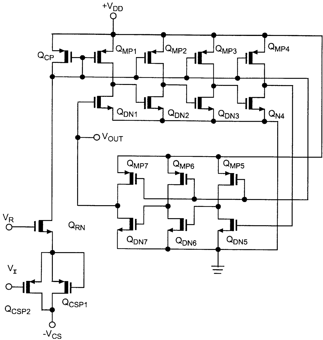
CMCMOS Ring Oscillator With NMOS Driver
