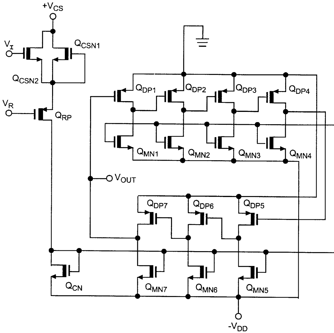
CCMOS Ring Oscillator With PMOS Driver
