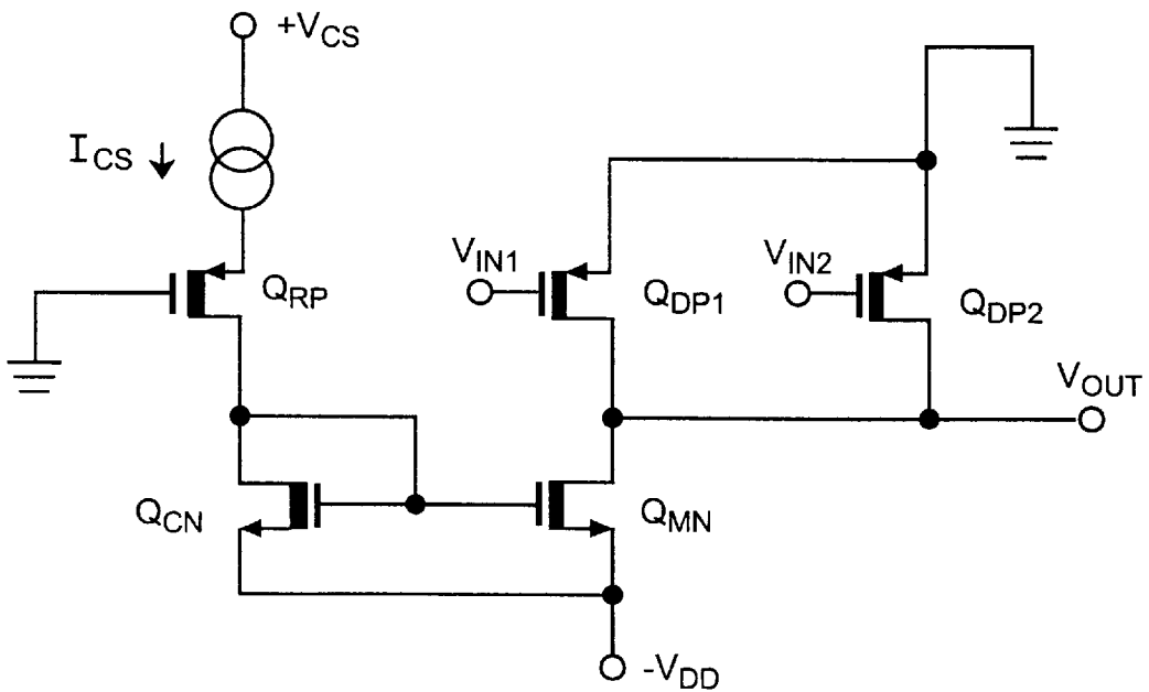
CMCMOS NOR Gate With PMOS Driver
