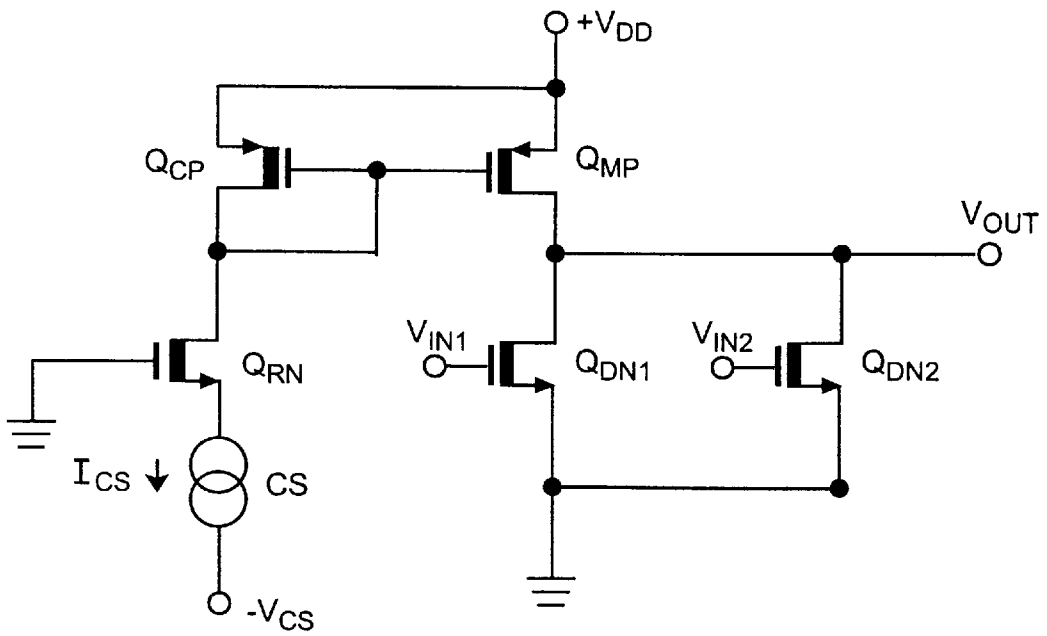
CMCMOS NOR Gate With NMOS Driver
