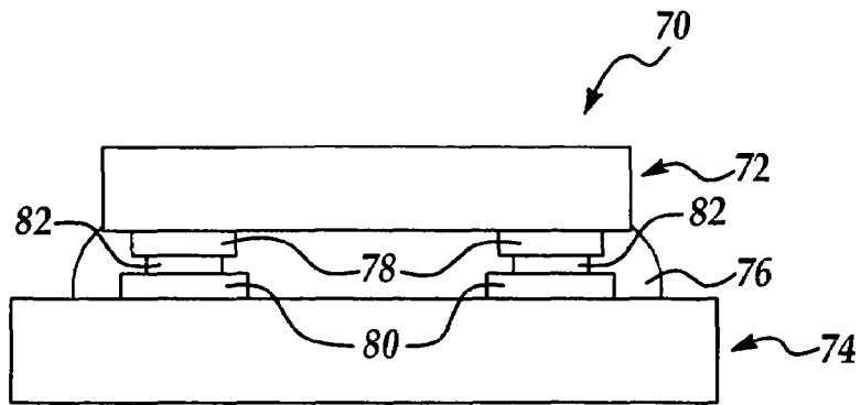
Figure 4A Prior Art
