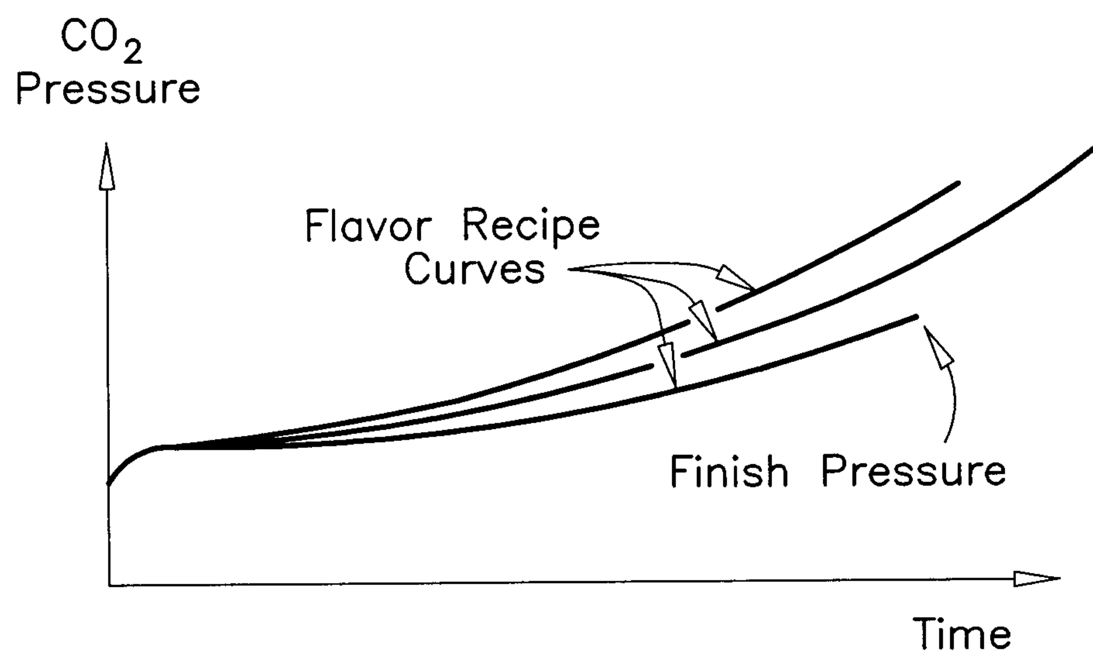
FIG. 2 PRIOR ART
