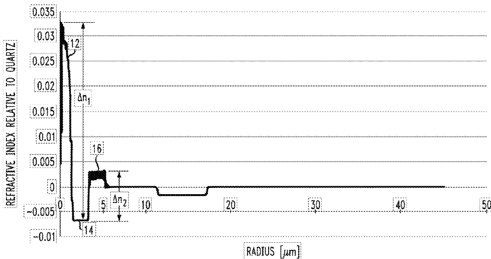
REFRACTIVE INDEX PROFILE
