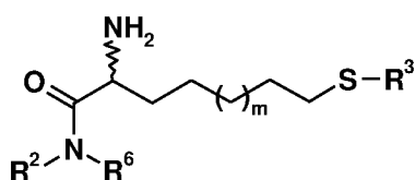
Formula III
