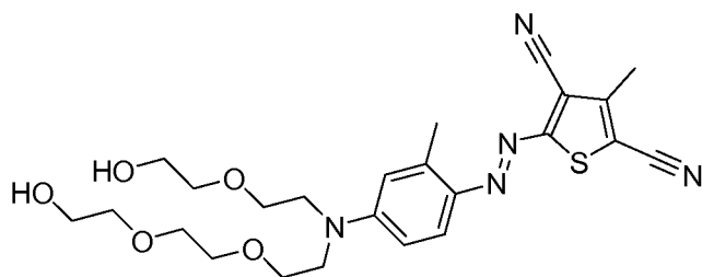
Compound 2
