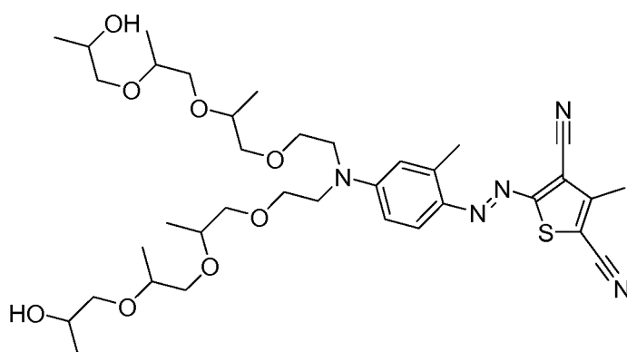
Compound 5
