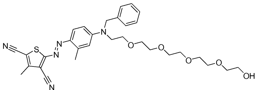
Compound 3
