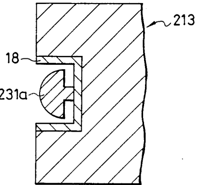
FIG. 5 PRIOR ART
