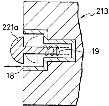
FIG. 3 PRIOR ART
