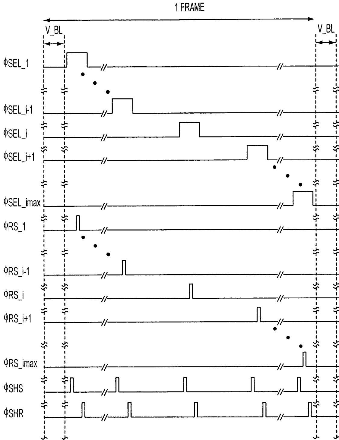
FIG. 3 PRIOR ART
