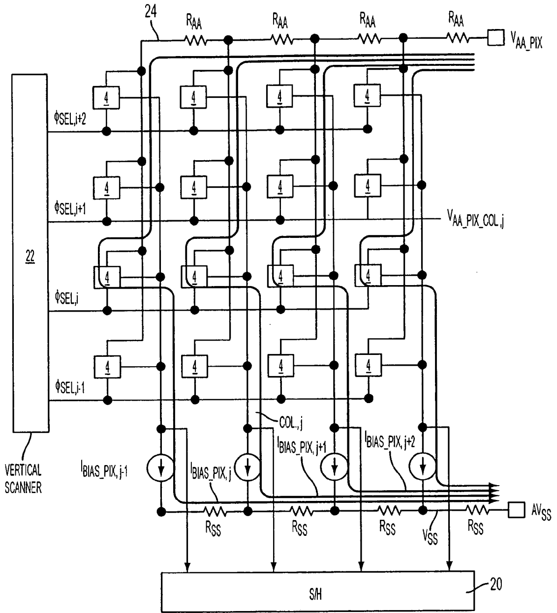
FIG. 4 PRIOR ART
