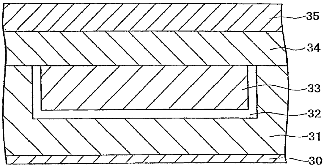
FIG. 12 (PRIOR ART)
