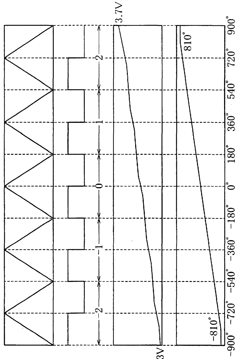
FIG. 45C OUTPUT OF DISPLACEMENT SENSOR
