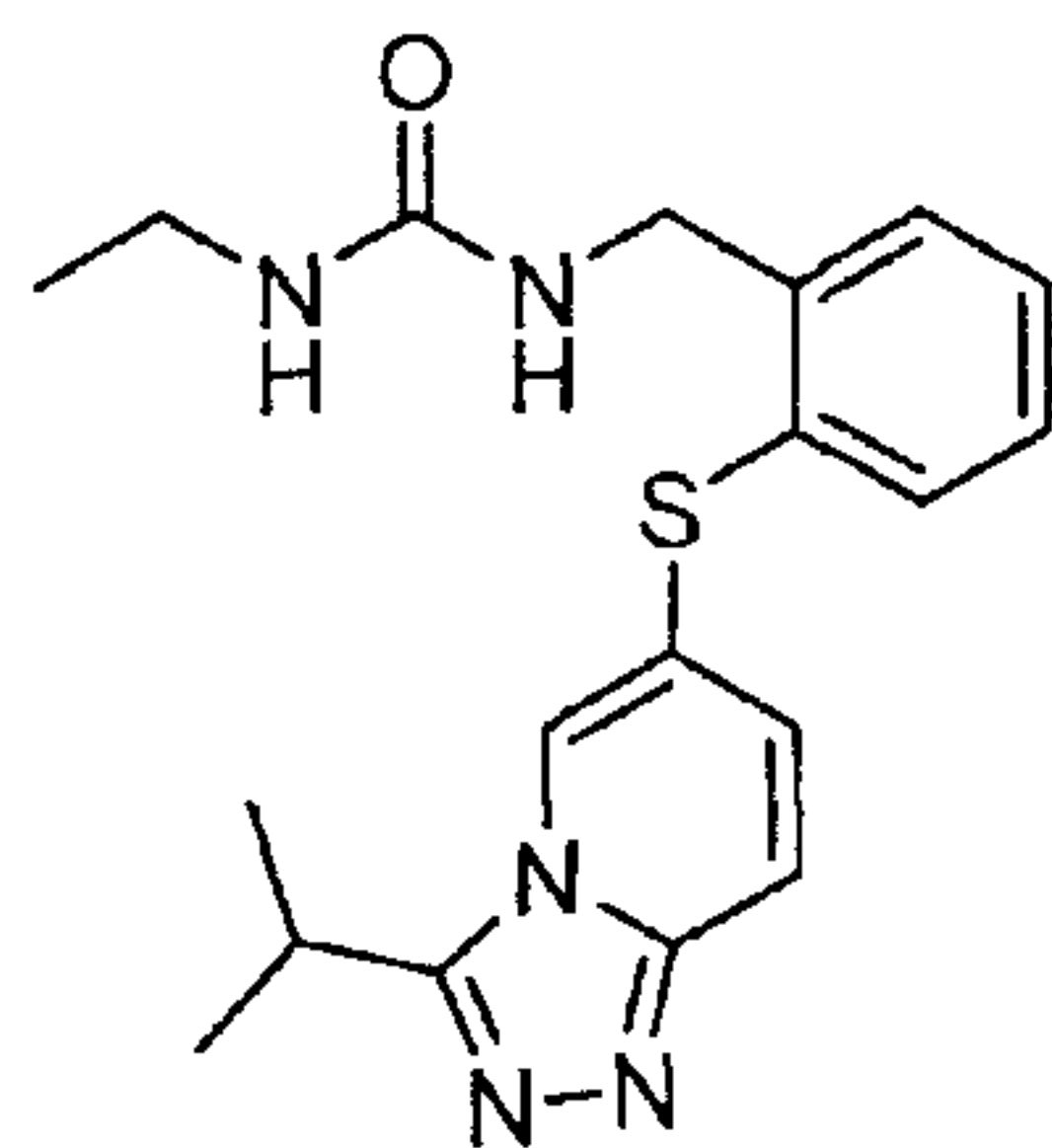
YIX (1-ethyl-3-(2-([3-(1-methylethyl)[1,2,4]triazolo[4,3-a]pyridine-6-yl)sulfanyl}benzyl)urea
