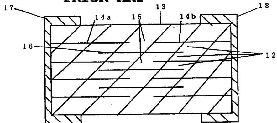
FIG. 8 PRIOR ART
