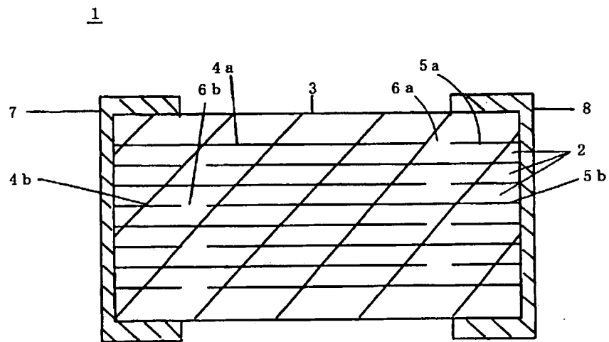
FIG. 7 PRIOR ART
