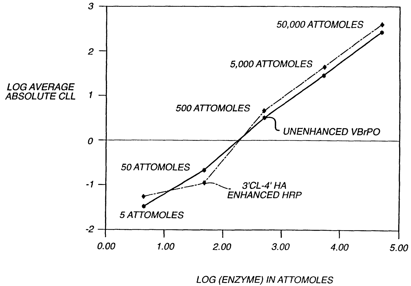
FIG. 1 ENHANCED HRP VS. UNENHANCED VBrPO; (ABSOLUTE CL SIGNAL)
