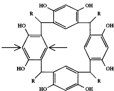
Phloroglucide
