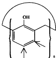
Calix [8] arene
