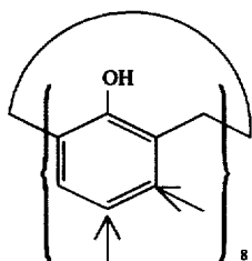
Alkyl-octols
