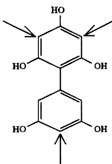
Phloroglucide
