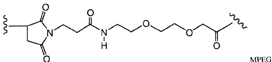
MP
