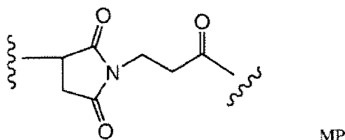
MP
