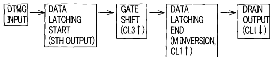
SEQUENCE OF THE LIQUID CRYSTAL DRIVER (EXAMPLE)
