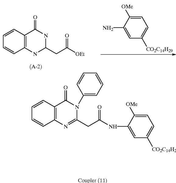
Coupler (11)
