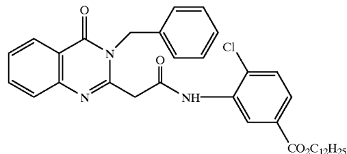
Coupler (10B)
