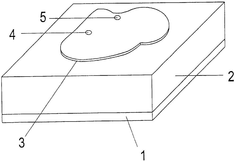
FIG. 8 PRIOR ART
