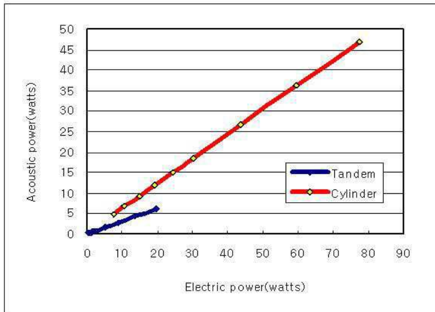
Fig 5. Acoustic power as a function of electric power applied
