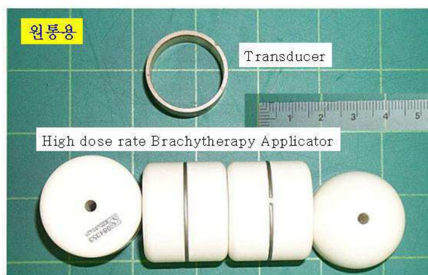
Fig 2. Picture of transducer which will be used as ultrasound source for cylindrical applicator
