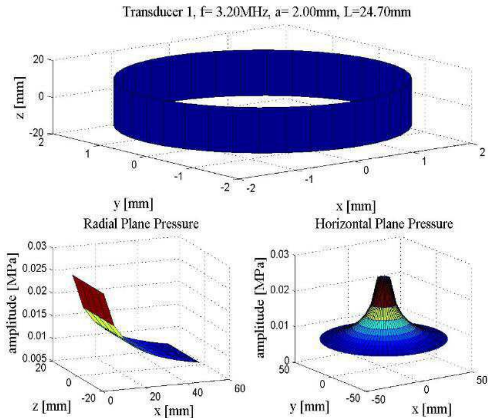
Fig 6. Calculated pressure field of tandem applicator
