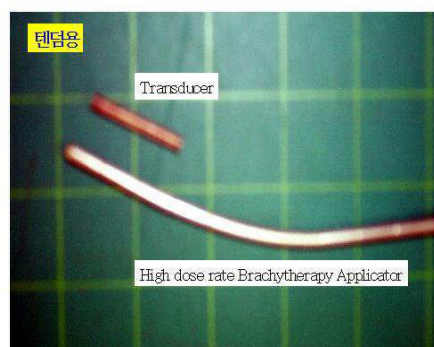
Fig 1. Picture of a transducer which will be used as a ultrasound source for tandem
