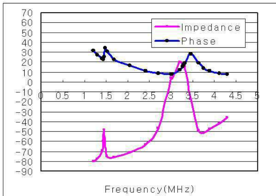
Fig 3. Magnitude and phase of the electrical impedance of the PZT-5A tube (OD=4mm, L=24.5mm) as a function of the operating frequency
