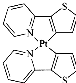
cis-Bis[2-(2'-thienyl)pyridinato-N,C 3 ] Pt (II) Pt(Thpy) 2
