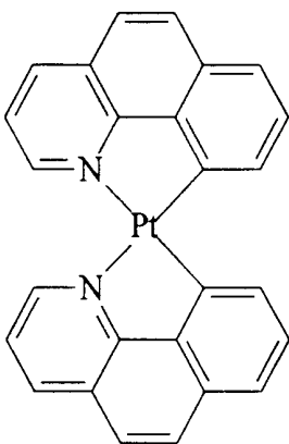
cis-Bis[2-(2-phenyl)pyridinato-N,C 2 ] Pt (II) Pt(Phpy) 2
