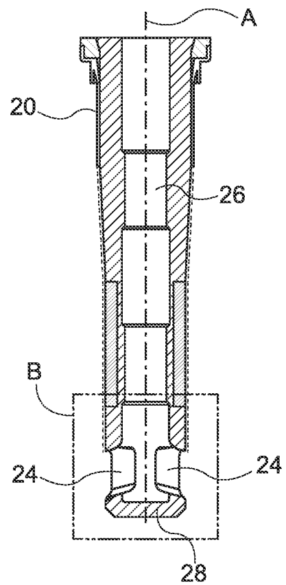
FIG. 3 (PRIOR ART)
