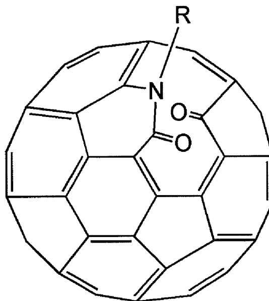
Molecule 1
