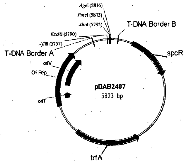
Figure 12: Schematic representation of plasmid pDAB2407
