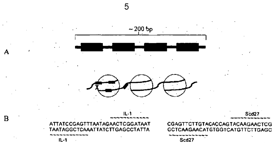
Figure 6: Zinc Finger Nuclease Binding Sequences and the Target Site Design for tobacco
