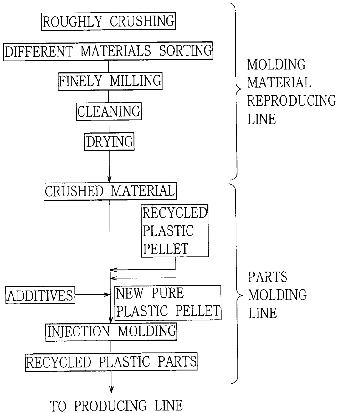
FIG. 3 SECOND PLASTIC RECYCLING LINE (NON-PELLETIZING LINE)
