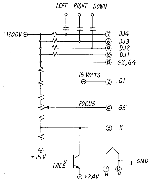
BIASING CIRCUITS - 3RPI FIG. 35
