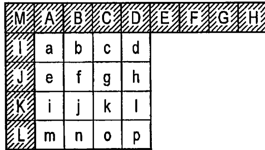
Arrangement of reference pixels and pixels to be encoded
