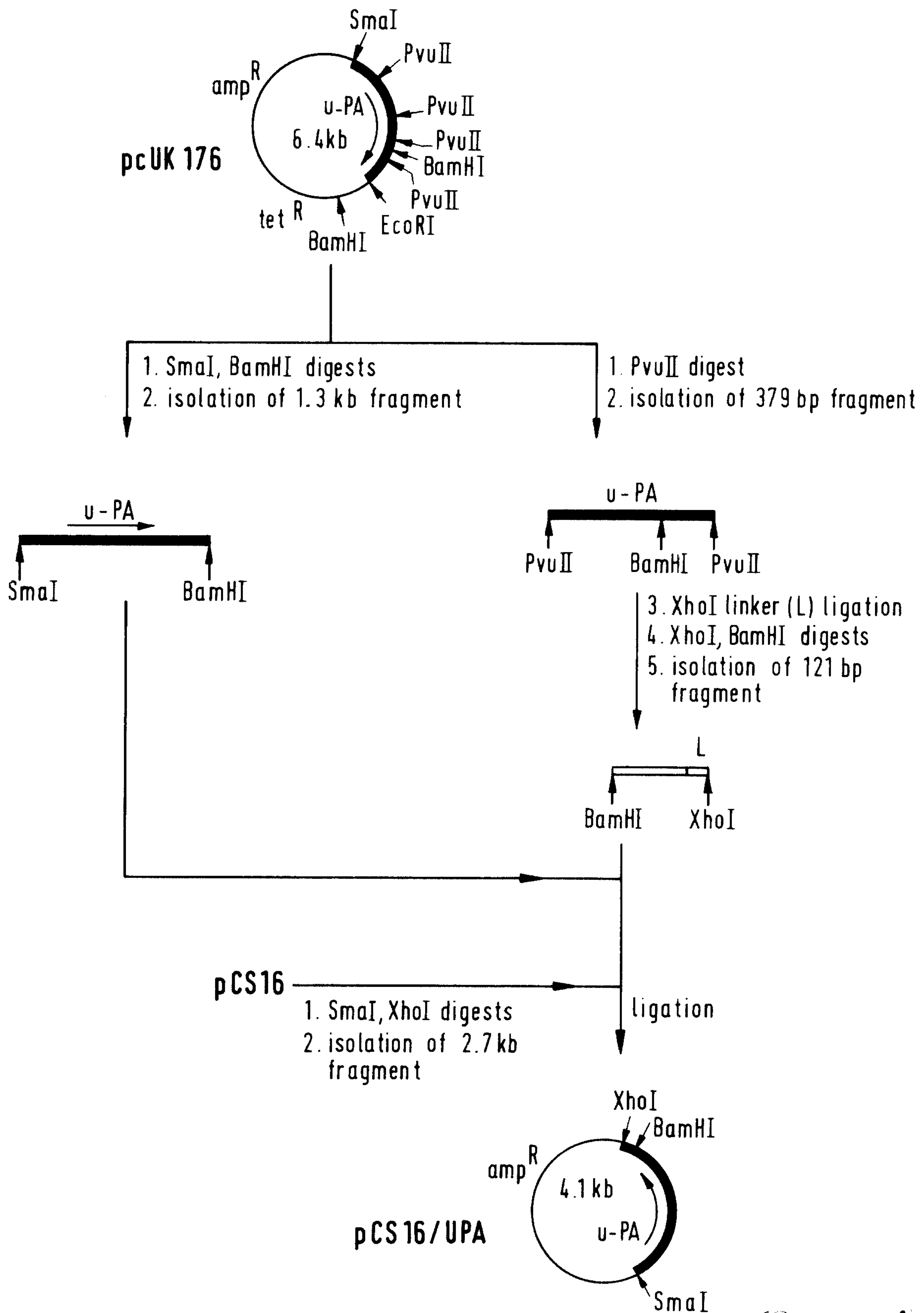
FIG. 4 : CONSTRUCTION OF PLASMID pCS16 / UPA
