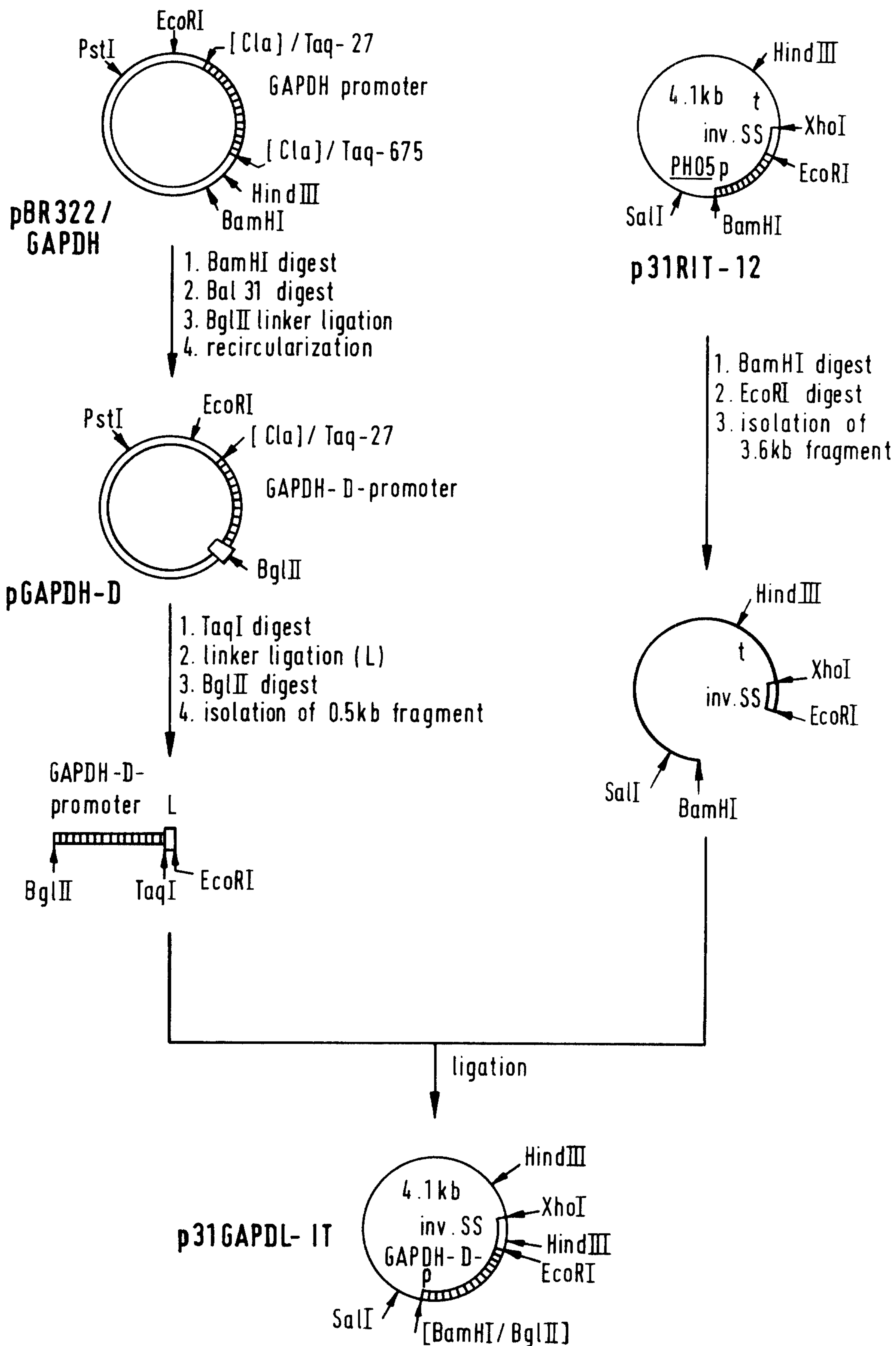
FIG.7: CONSTRUCTION OF PLASMID p31GAPDL-IT
