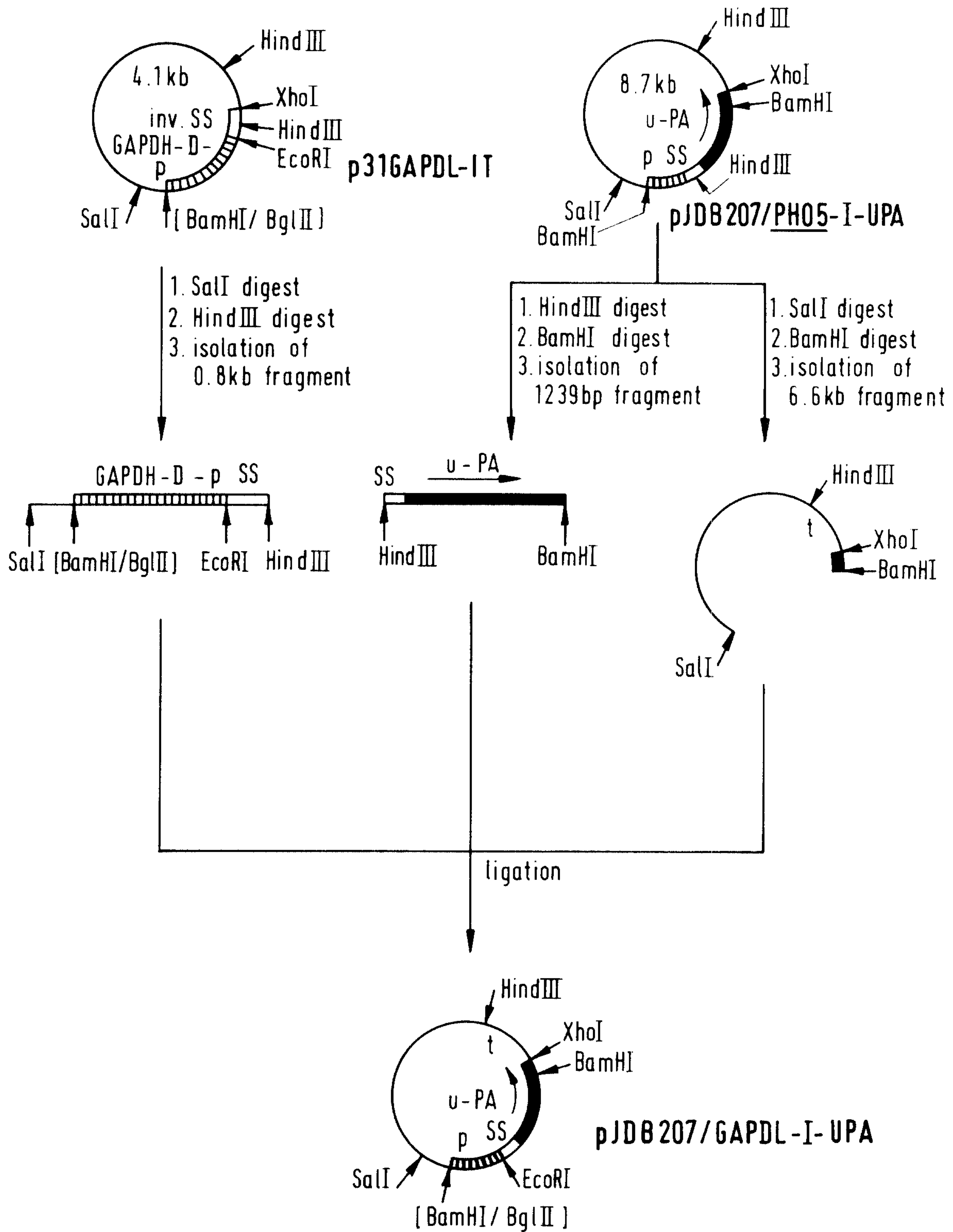
FIG.9 : CONSTRUCTION OF PLASMID pJDB207 / GAPDL-I- UPA
