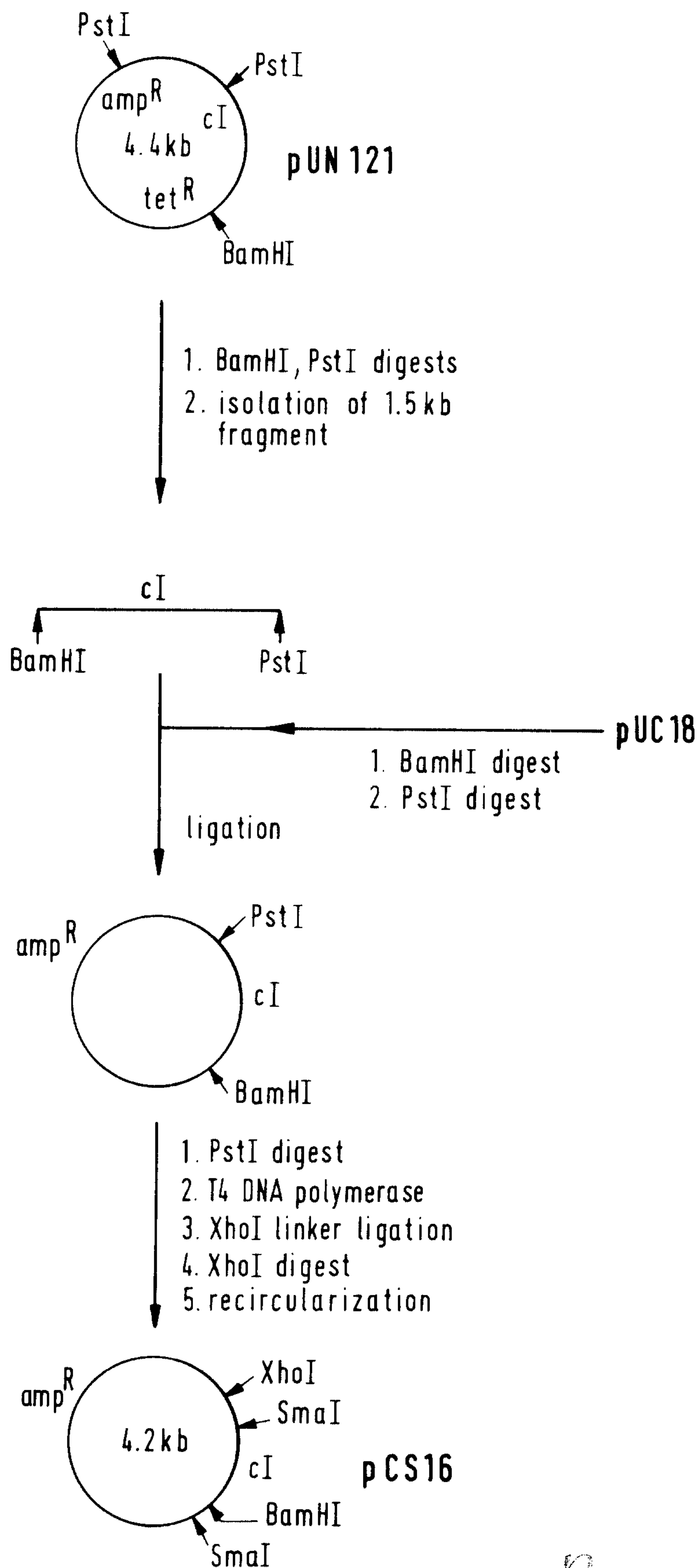
FIG.3 : CONSTRUCTION OF PLASMID pCS16
