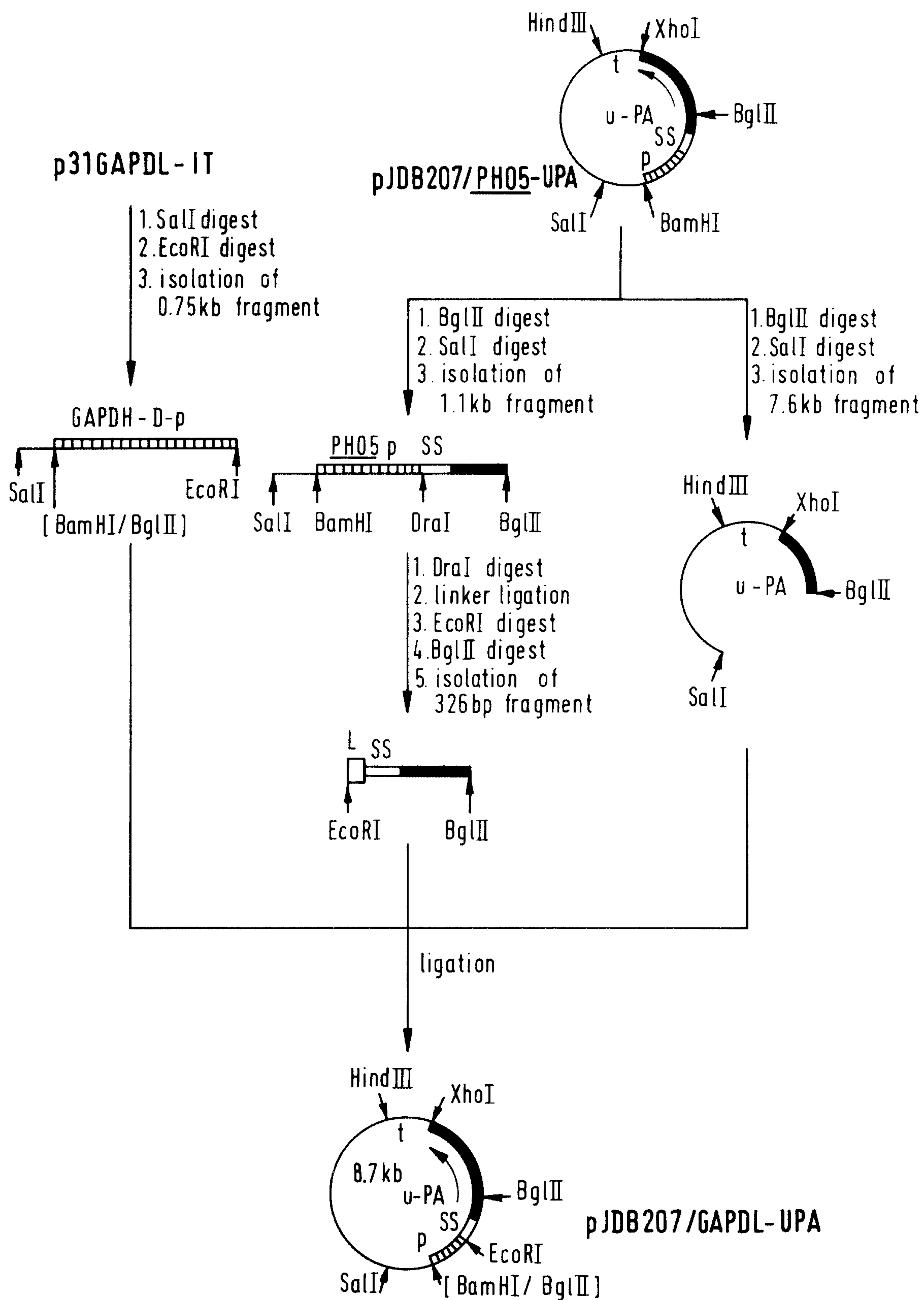
FIG.10 : CONSTRUCTION OF PLASMID pJDB207/ GAPDL- UPA
