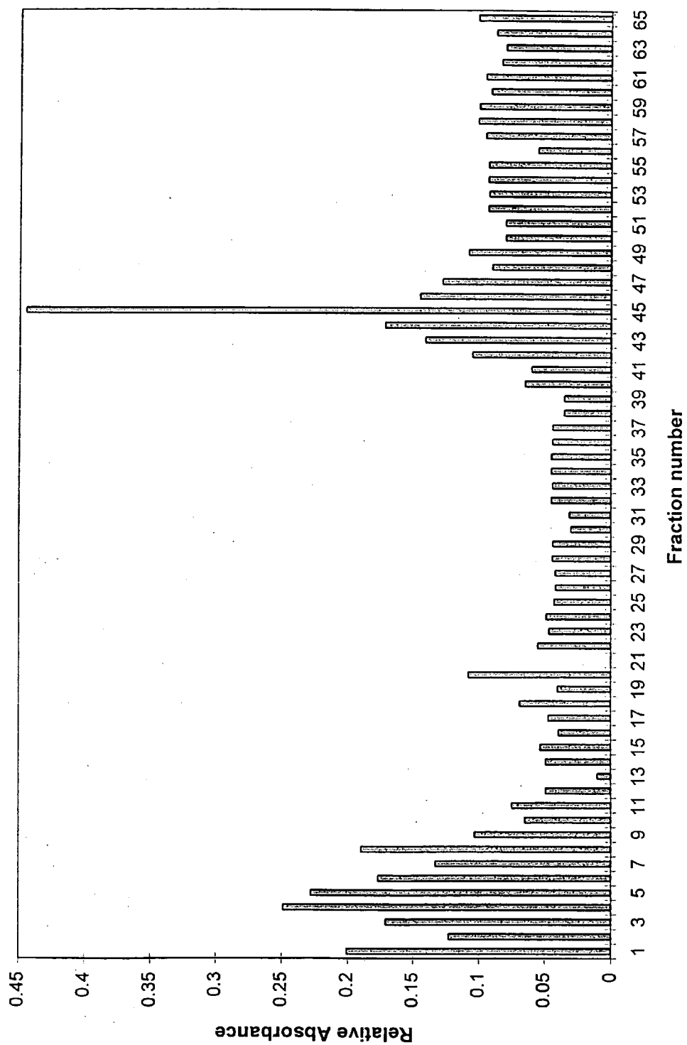
Elution profile of bovine serum albumin on tertiary amine fibril column
