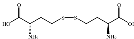
L-Homocystine MW 268.35 99.9 HI
