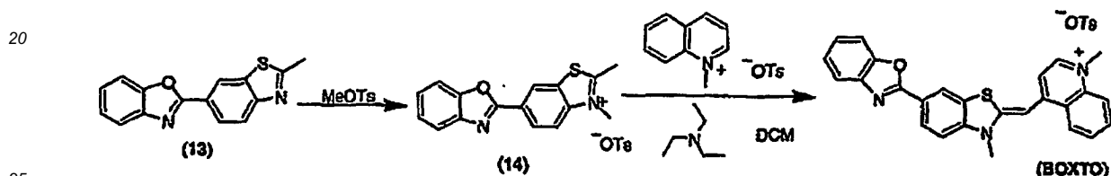
Scheme 9. The two final steps in the synthesis of BOXTO.
