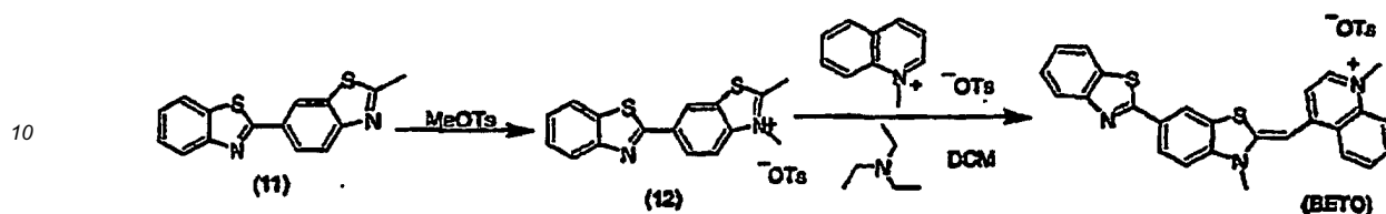
Scheme 8. The two final steps in the synthesis of BETO.
