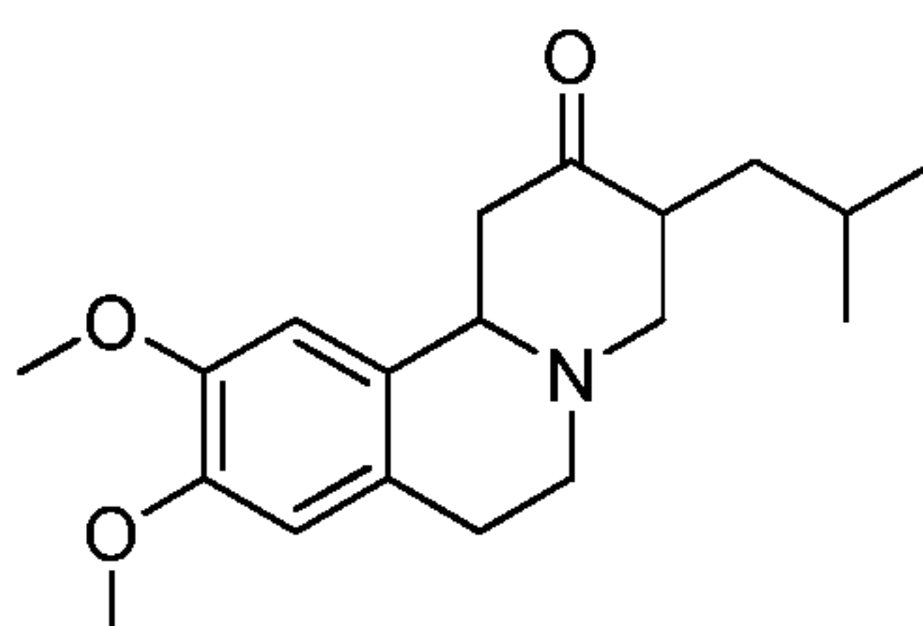
Tetrabenazine
